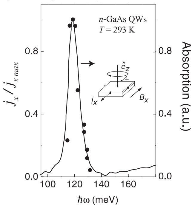
Figure 20. The spectral dependence of the spin-galvanic effect for (001)-grown n-type GaAs QWs of 8.2 nm width at room temperature. Data (dots) are presented for optical excitation by normally incident right-handed circularly polarized radiation. A magnetic field of B_x = 1 T was used. For comparison the absorption spectrum is shown, by the full curve.
